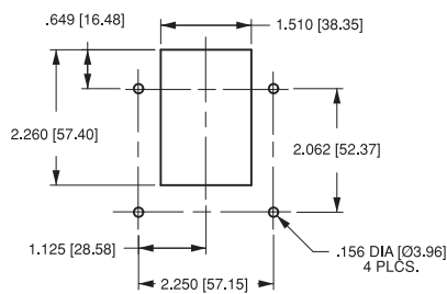
PANEL CUT-OUT DETAIL
