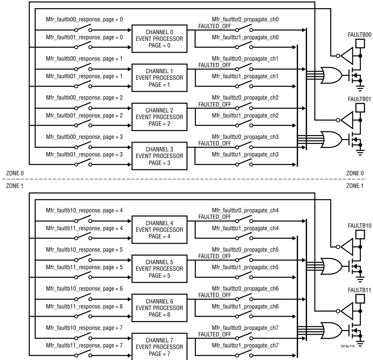
Figure 19. Channel Fault Management Block Diagram
