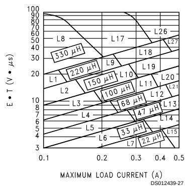
FIGURE 7. LM2594/LM2594HV-ADJ
