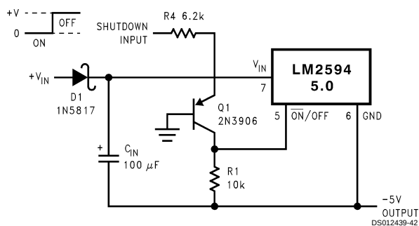
FIGURE 27. Inverting Regulator Ground Referenced Shutdown
