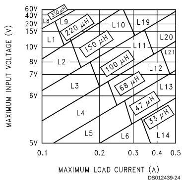
FIGURE 4. LM2594/LM2594HV-3.3
