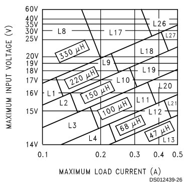
FIGURE 6. LM2594/LM2594HV-12
