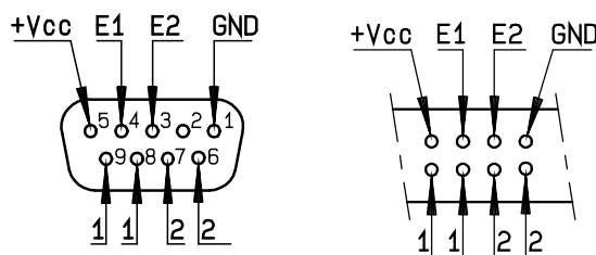
D-Sub connector
