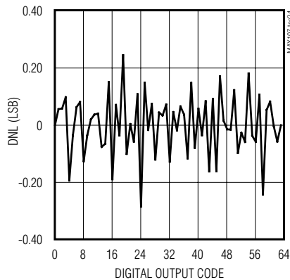
DNL vs. DIGITAL OUTPUT CODE
