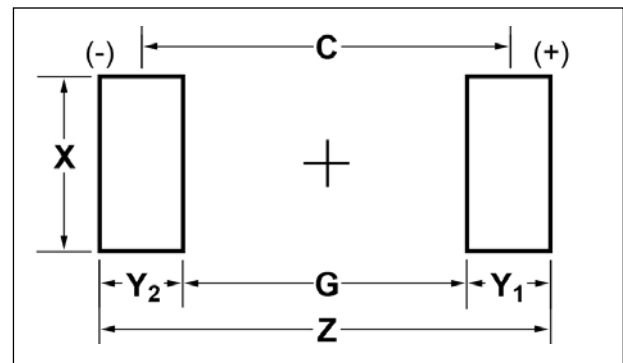
T528I & M Pad Dimensions (mm)
