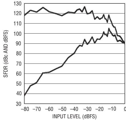
LTC2206: SFDR vs Input Level, f_{IN} = 140.2\text{MHz} , PGA = 0, Dither "On", 80Mps
