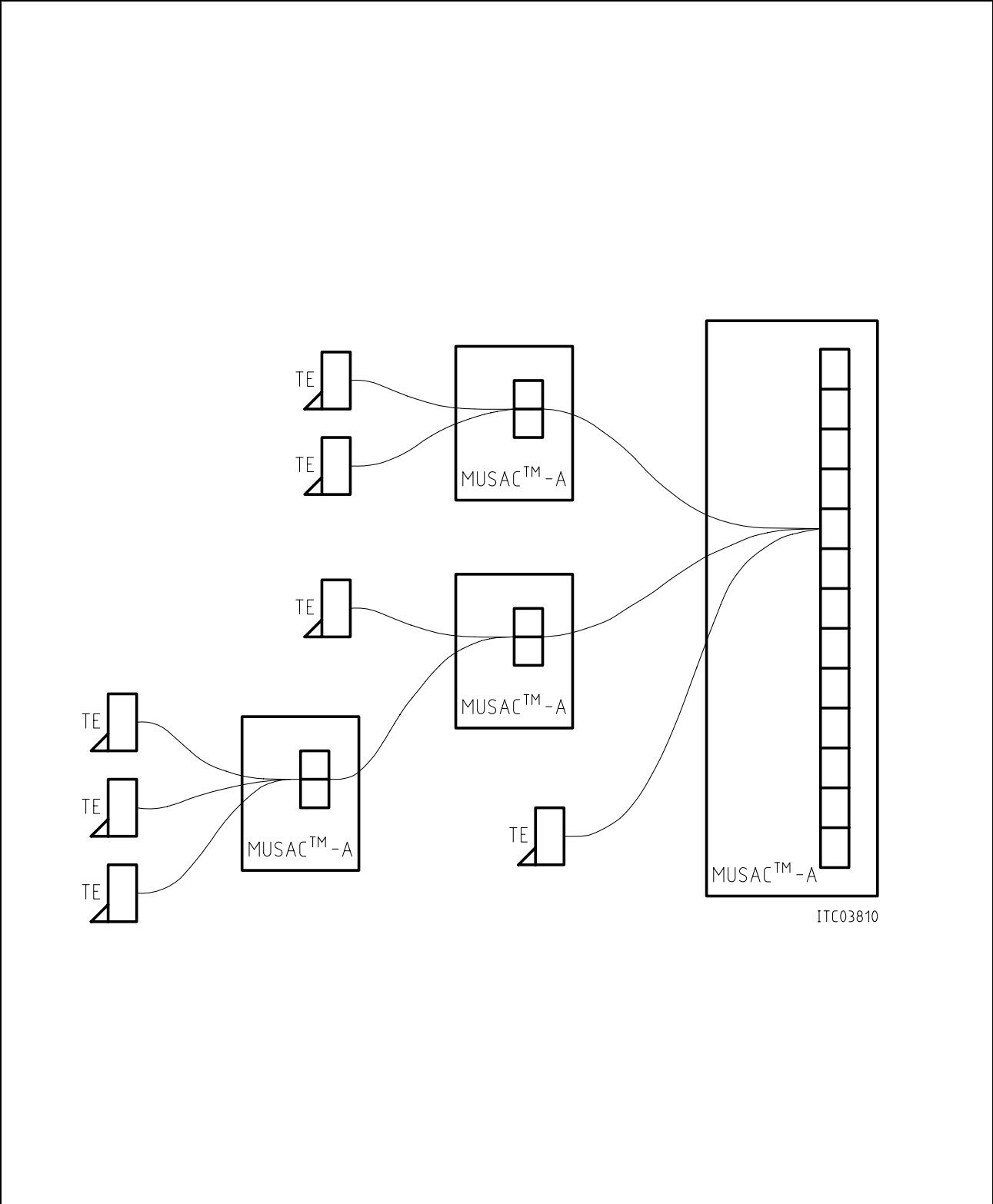
Figure 10 Multistage Arrangement
