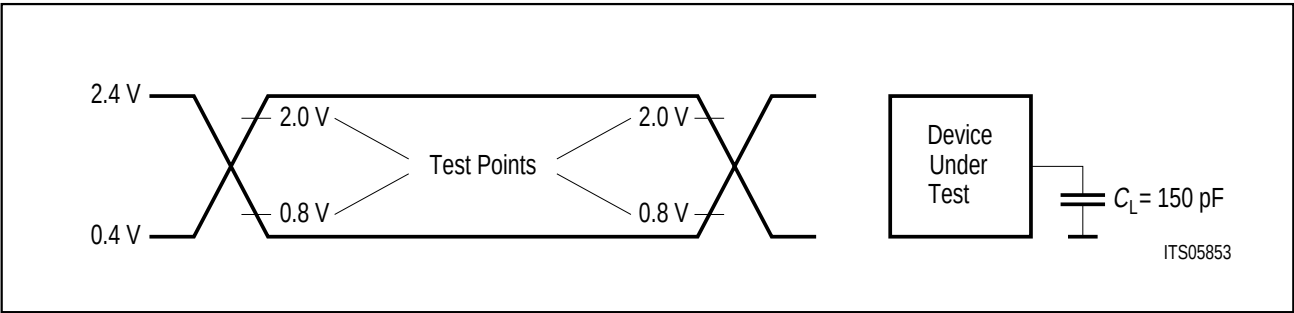
Figure 21 I/O-Wave Form for AC-Test
