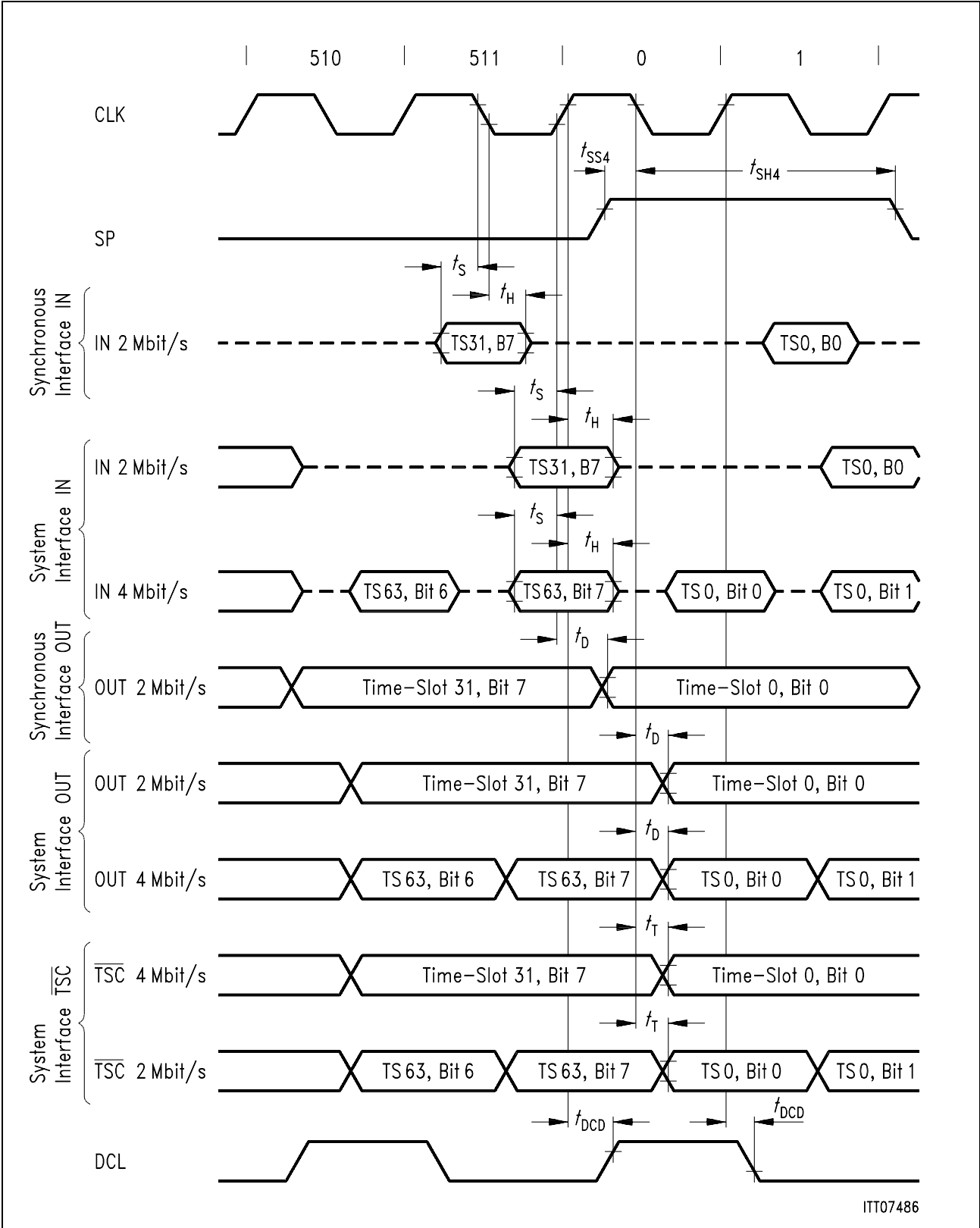
Figure 29 PCM Line Timing in Primary Access Configuration with a 4 MHz Device Clock and a CSR Entry (00010001)
