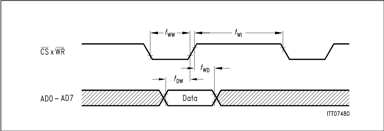
Figure 23 \mu P Write Cycle
