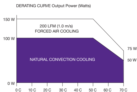
Figure 1: Derating Curve
