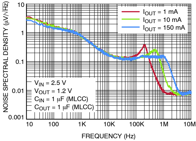
Figure 21. Output Voltage Noise Spectral Density – V_{\text{OUT}} = 1.2 \text{ V}
