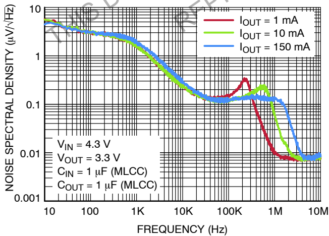
Figure 23. Output Voltage Noise Spectral Density – V_{\text{OUT}} = 3.3 \text{ V}
