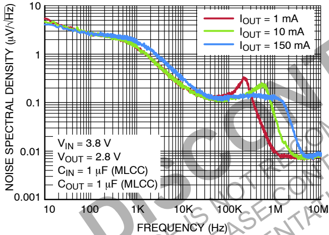
Figure 22. Output Voltage Noise Spectral Density – V_{\text{OUT}} = 2.8 \text{ V}
