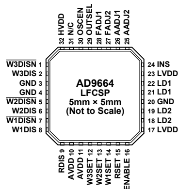
Figure 2. 4-Channel LVDS Laser Driver Pin Configuration
