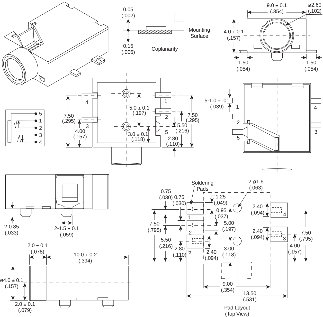
Dimensions mm and (In.)
