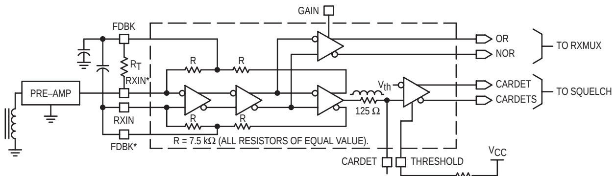
Figure 4–1. Receiver Amplifier With Carrier Detect
