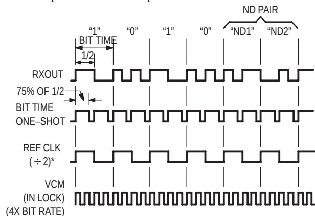
Figure 5–2. Clock Recovery Timing Signals
