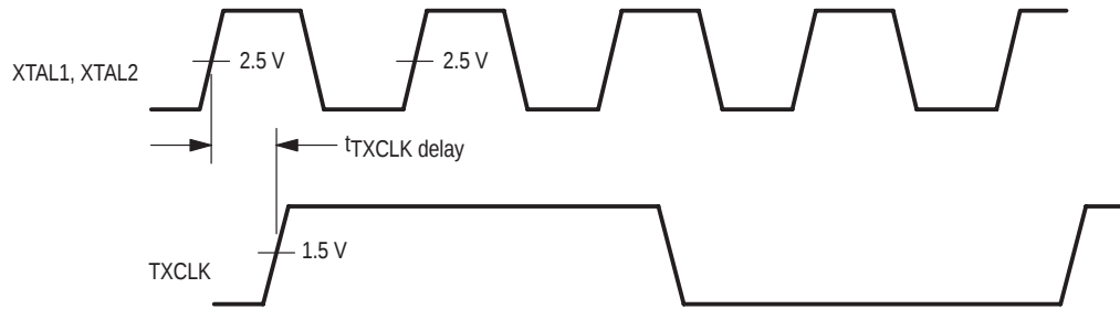
(C) TXCLK Delay Timing to XTAL1, XTAL2
