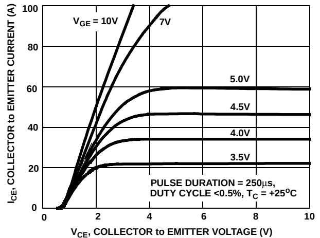
FIGURE 2. SATURATION CHARACTERISTICS
