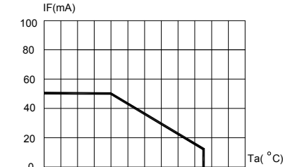
FIG.4a RED MAXIMUM FORWARD DC CURRENT VS AMBIENT TEMPERATURE ( T_{jmax}=105^{\circ}C )
