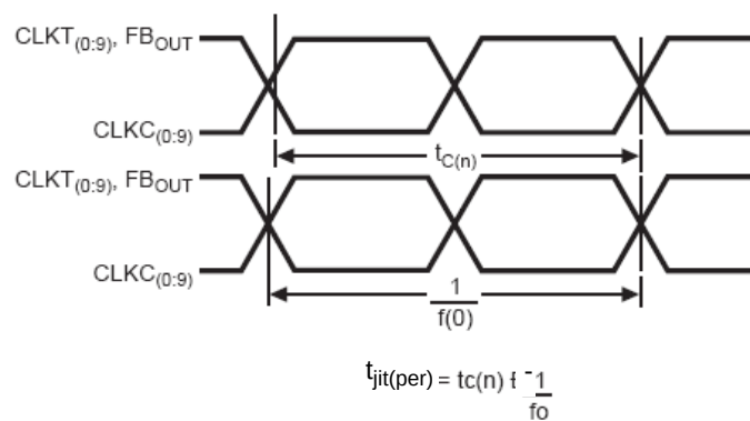
Figure 3. Period Jitter
