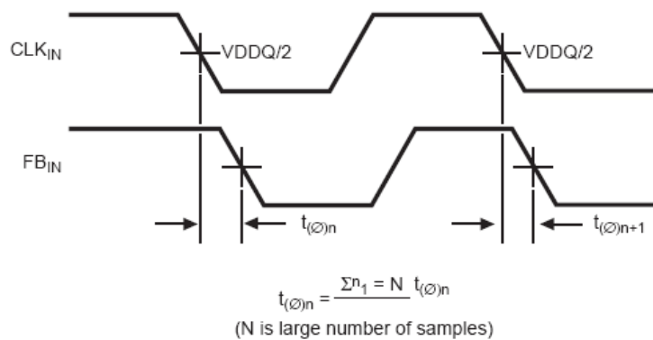
Figure 5. Static Phase Offset (Differential Probes)
