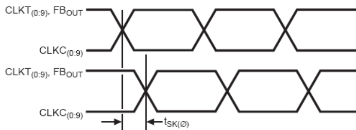
Figure 7. Output Skew
