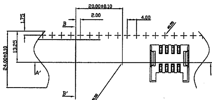
DETAIL X
