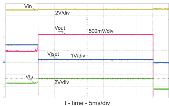
Figure 8-5. Battery Removal – GND Removed 1st, 42-Ω Load
