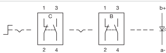
Wiring diagram 286
