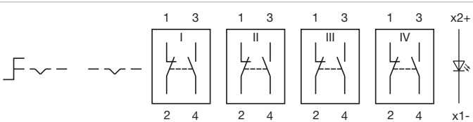
Wiring diagram 280
