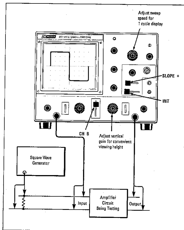
Fig. 28. Equipment set-up for square-wave testing of amplifiers.
