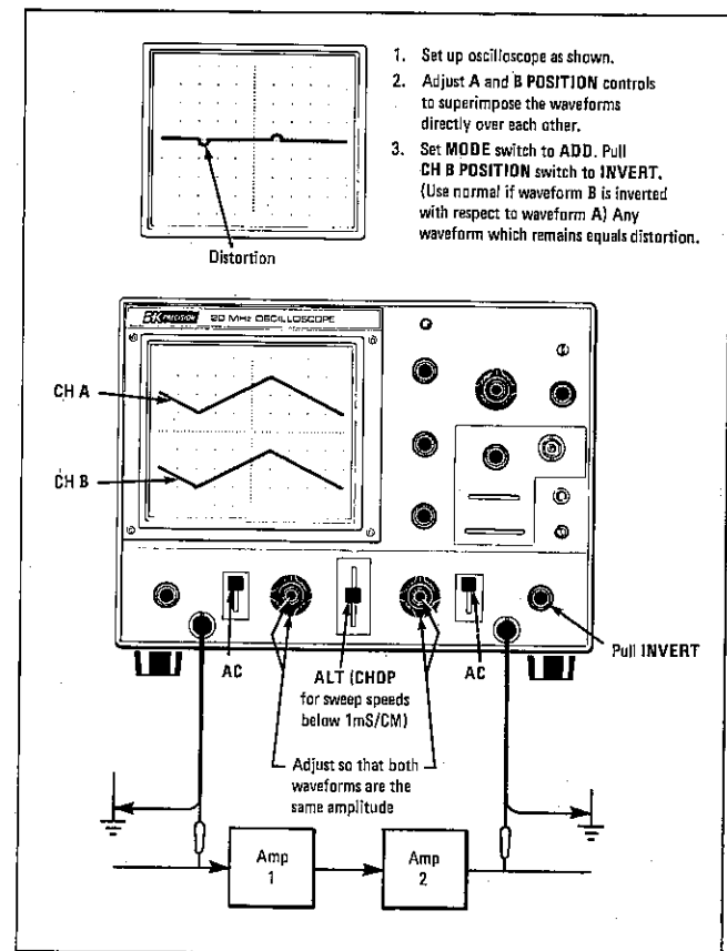
Fig. 14. Distortion measurement.
