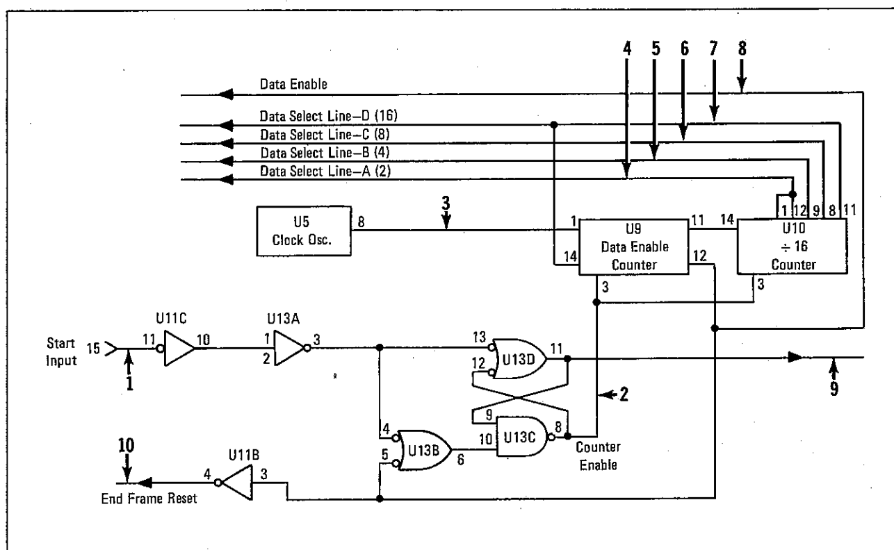
Fig. 12. Typical digital circuit using several time-related waveforms.
