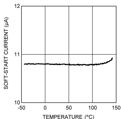
Figure 6-9. Soft Start vs Temperature
