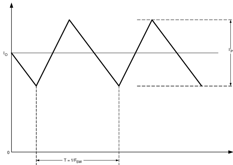
Figure 8-2. Inductor Current
