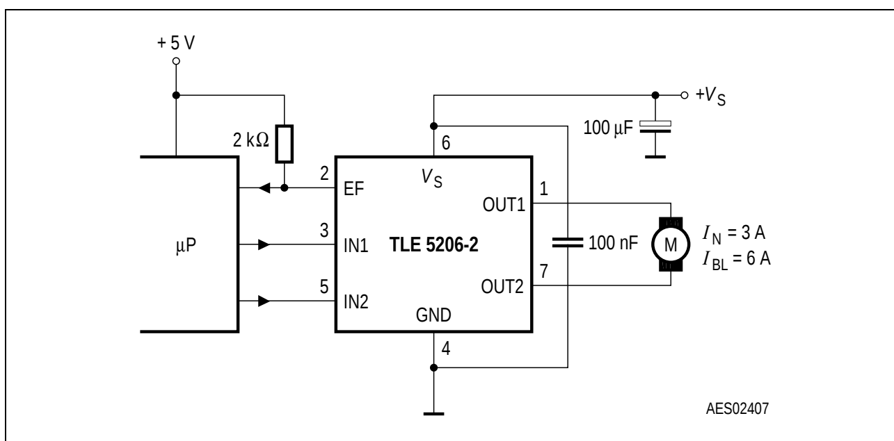
Figure 5 Application Circuit
