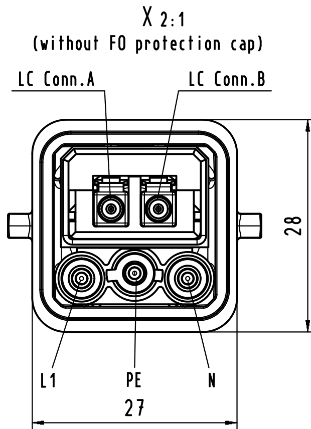
Hybrid Han 3A - LC Duplex and Power AC, with metal housing
