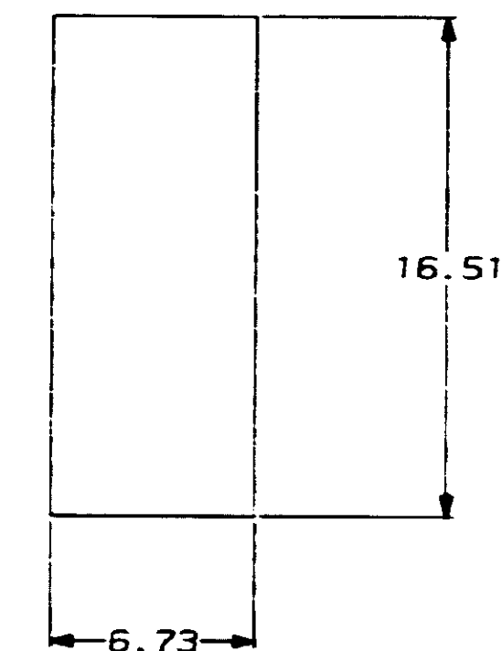
RECOMMENDED CUT OUT FOR 1.52 MAX THICK PANEL
