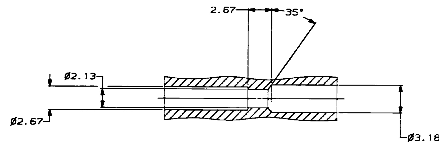
TYPICAL RECEPTACLE CAVITY SECTION (DIMENSIONS REFERENCE ONLY)
