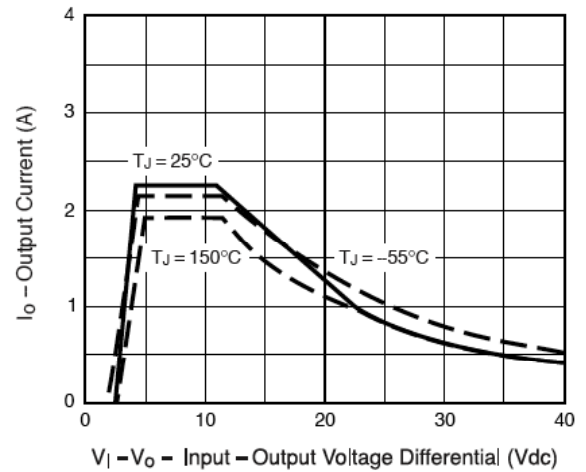
Figure 6. Current Limit
