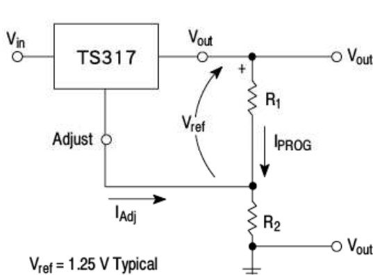
Figure 17. Basic Circuit Configuration
