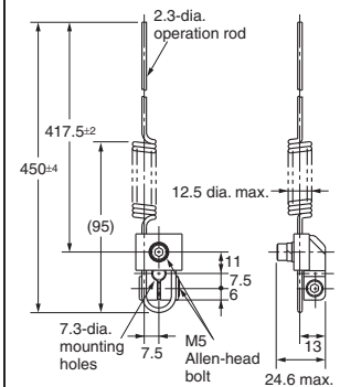
WL-5A101
