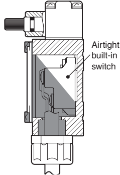
WLG□-RP40
