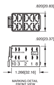
VC1 CONNECTOR HOUSING
