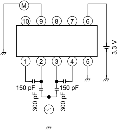
(a) DIFF-AMP CMRR
