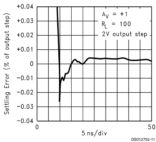
Settling Time
