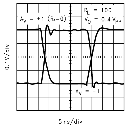
Pulse Response
