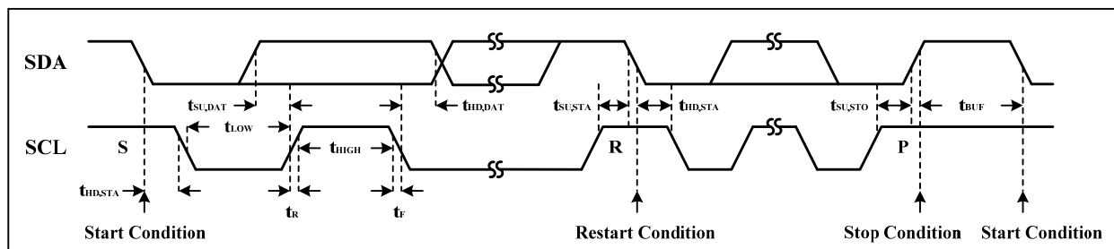
Figure 3 Interface timing
