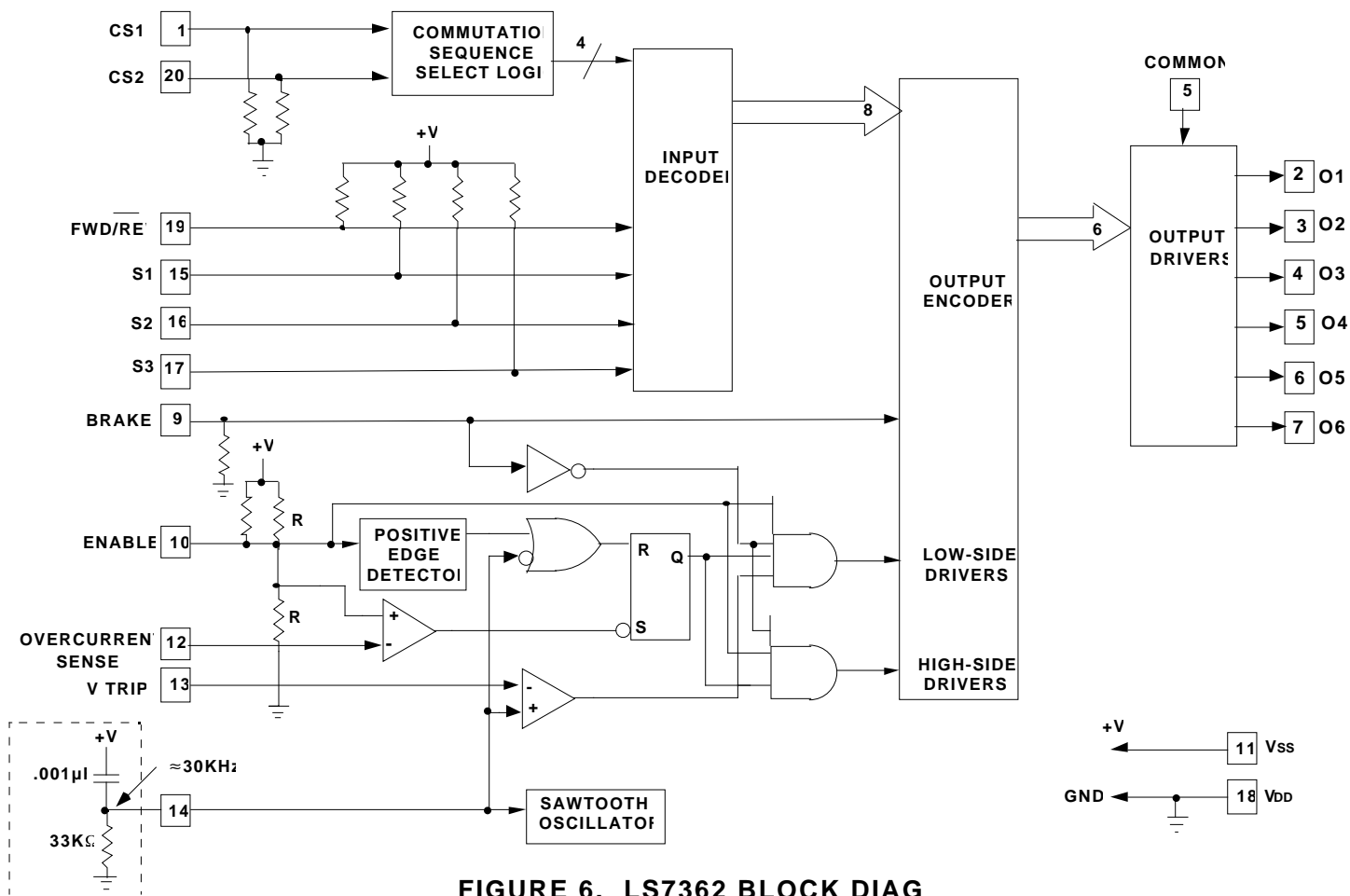
FIGURE 6. LS7362 BLOCK DIAG
