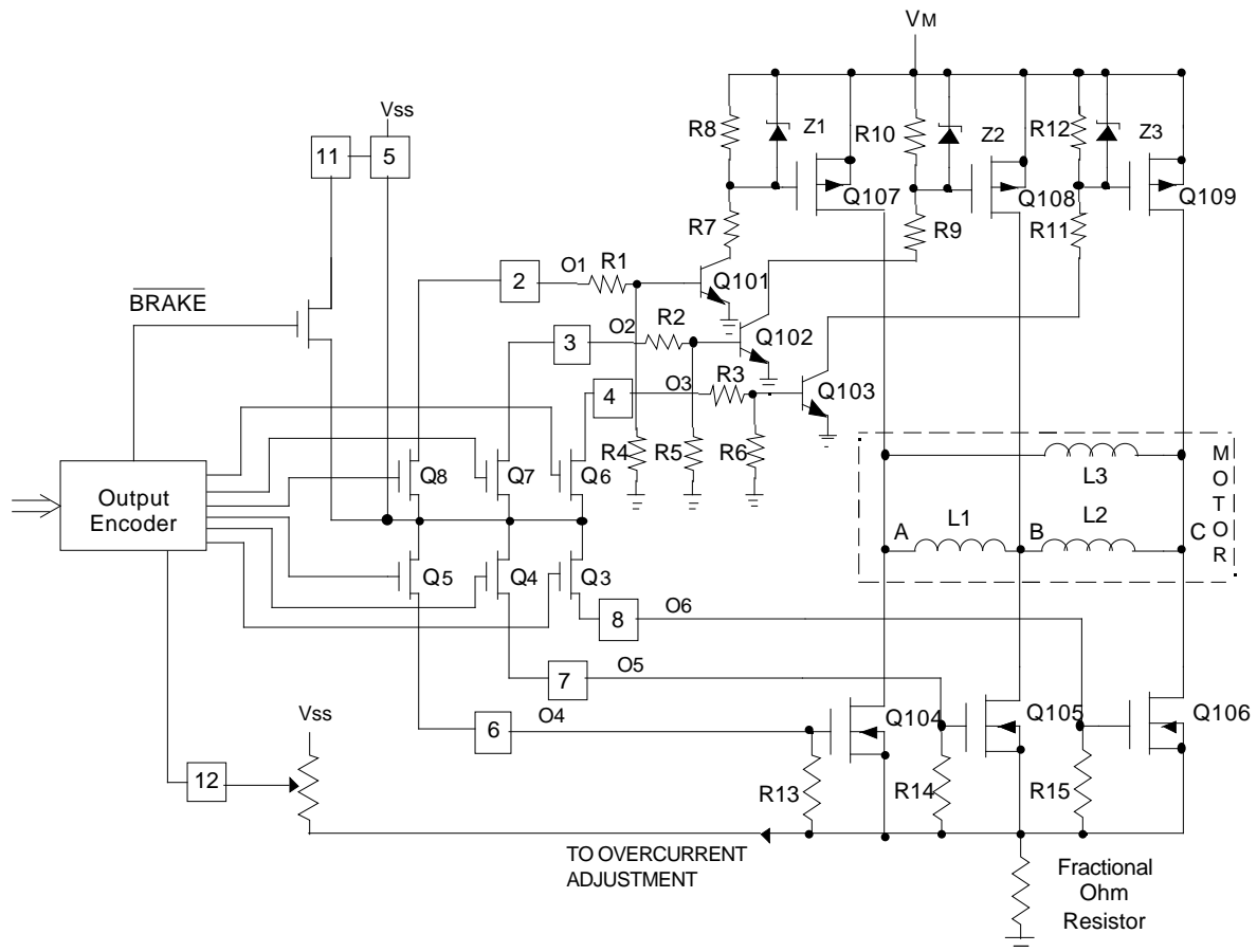
FIGURE 2. POWER FET THREE PHASE OUTPUT DRIVER CIRCUITRY
