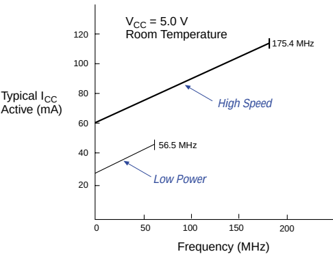
EPM7064S
