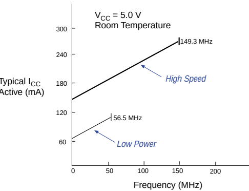
EPM7160S
