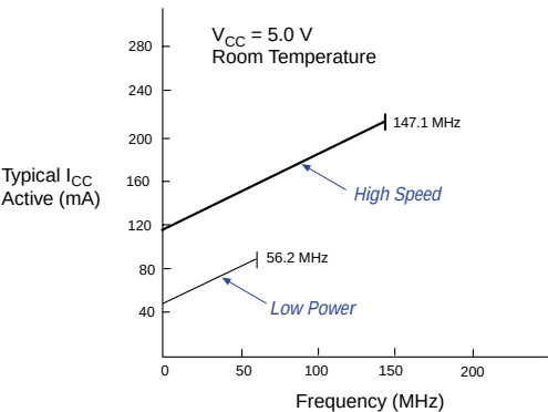
EPM7128S
