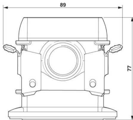
Dimensional drawing
