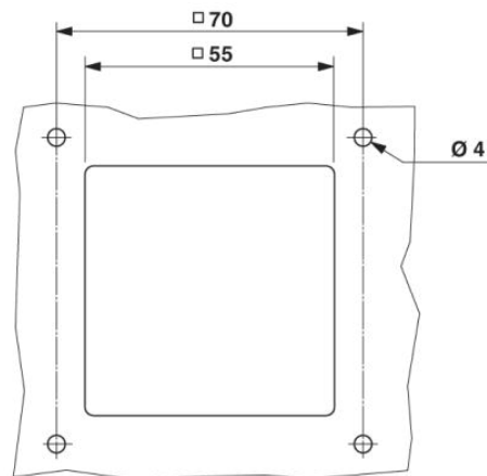
Panel cutout: DC-B 6-HB-M
