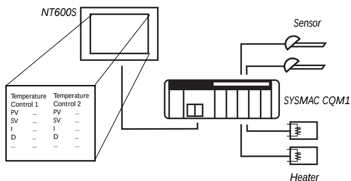
Host Link Application
