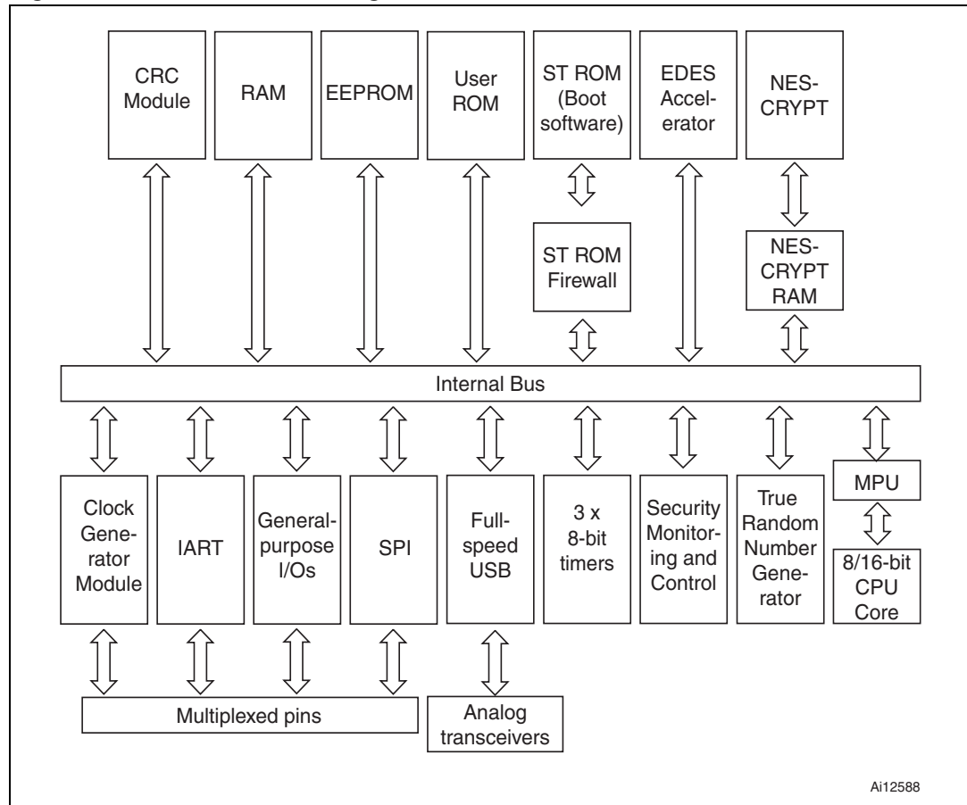
Figure 1. ST23YT66 block diagram
