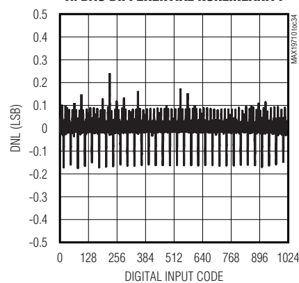
Tx DAC DIFFERENTIAL NONLINEARITY
