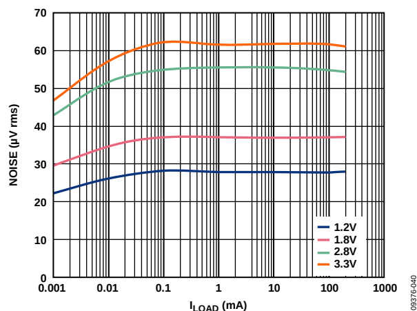
Figure 60. RMS Output Noise vs. Load Current and Output Voltage, V_{IN} = 5\text{ V} , C_{OUT} = 1\text{ μF}
