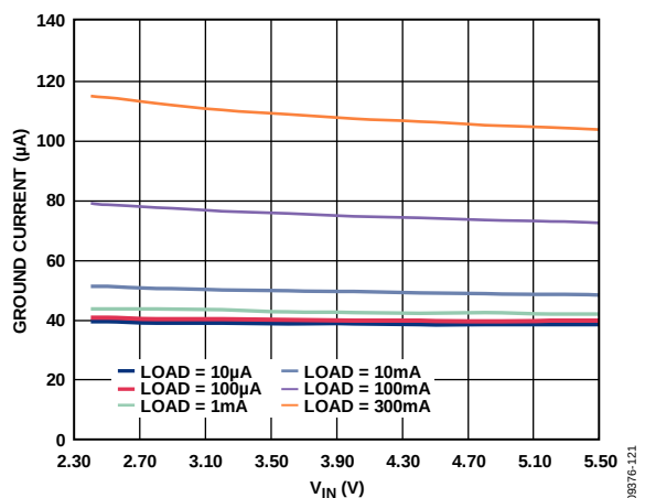
Figure 21. Ground Current vs. Input Voltage, V_{OUTx} = 1.2V , ADP222/ADP224
