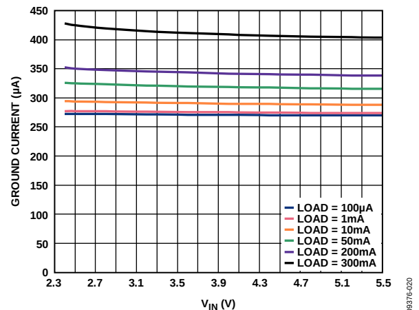
Figure 40. Ground Current vs. Input Voltage, V_{OUTx} = 1.2 V and 1.8 V, Dual Output, Includes 200 \mu A for Output Dividers, ADP223/ADP225
