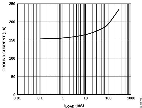
Figure 37. Ground Current vs. Load Current, Single Output, Includes 100 \mu A for Output Divider, ADP223/ADP225
