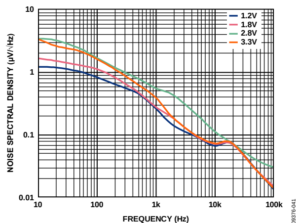
Figure 61. Output Noise Spectral Density, V_{IN} = 5\text{ V} , I_{LOAD} = 10\text{ mA} , C_{OUT} = 1\text{ μF}
