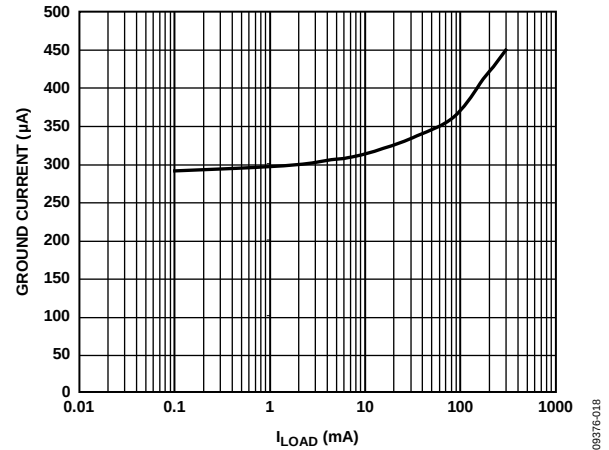
Figure 38. Ground Current vs. Load Current, Dual Output, Includes 200 \mu A for Output Dividers, ADP223/ADP225
