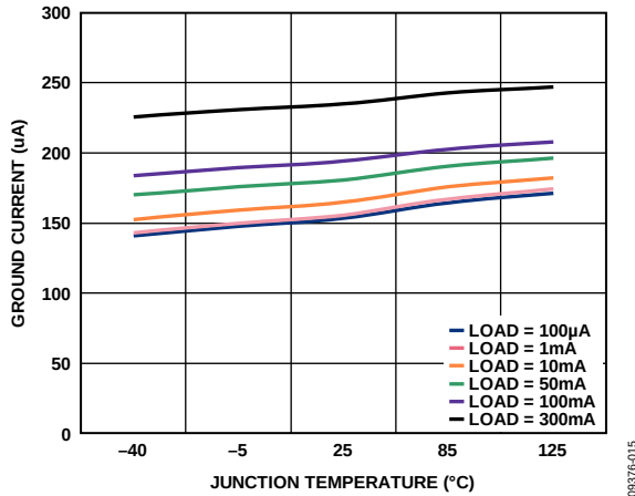
Figure 35. Ground Current vs. Junction Temperature, Single Output, Includes 100 \mu A for Output Divider, ADP223/ADP225
