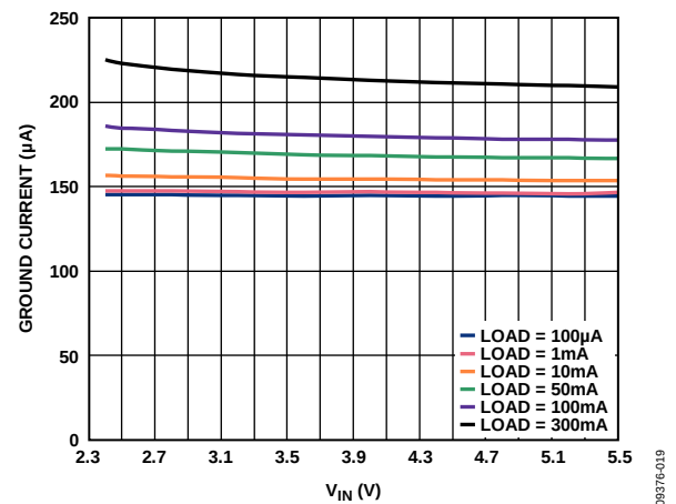
Figure 39. Ground Current vs. Input Voltage, V_{OUTx} = 1.2 V, Single Output, Includes 100 \mu A for Output Divider, ADP223/ADP225
