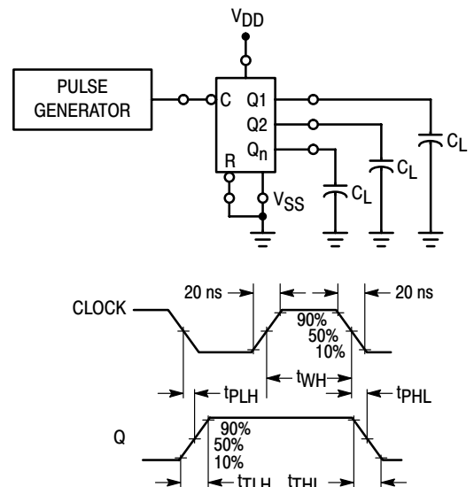
Figure 2. Switching Time Test Circuit and Waveforms
