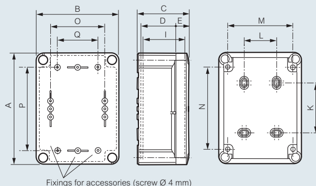
Fixings for accessories (screw Ø 4 mm)
