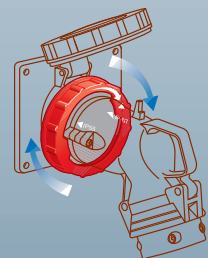
IP 66/67-55 obtained with locking ring secured
