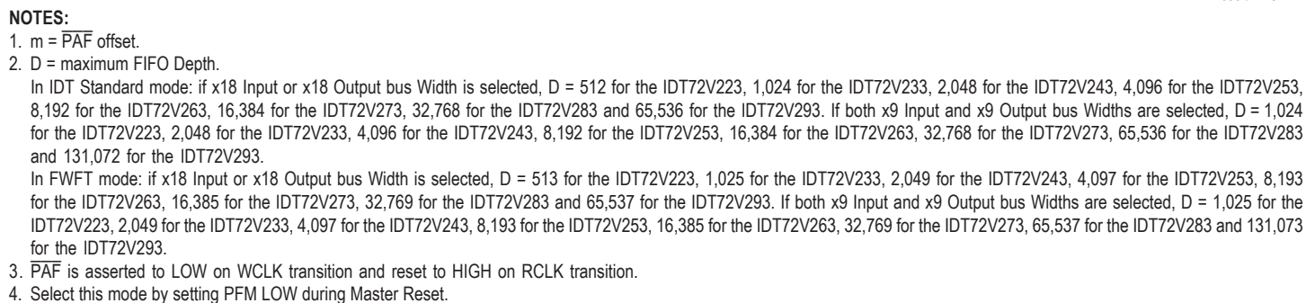
Figure 20. Asynchronous Programmable Almost-Full Flag Timing (IDT Standard and FWFT Modes)
