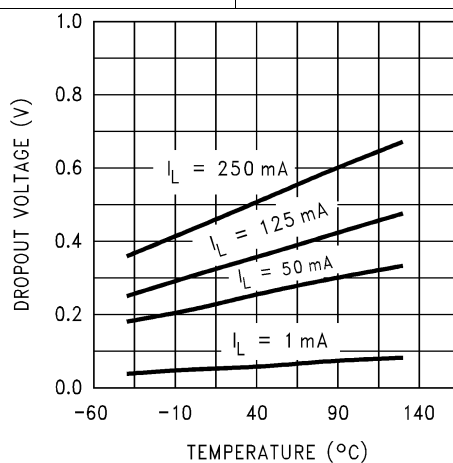
Figure 27. Dropout Voltage
