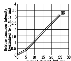
Fig4. RELATIVE LUMINOUS INTENSITY VS. FORWARD CURRENT
