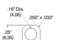
S 3 Solder Eye, extra large & quick connect
