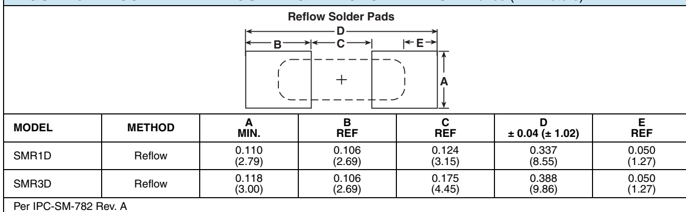
FIGURE 3 - RECOMMENDED MOUNTING PAD GEOMETRIES in inches (millimeters)
