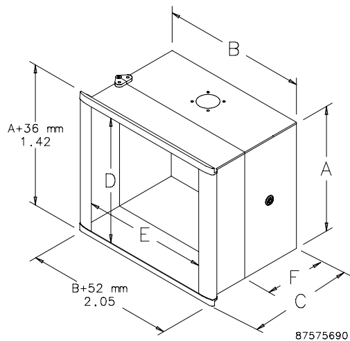
Hinged Enclosure
