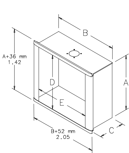
Solid Enclosure
