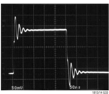
Small-Signal Transient ( A_V = 1 , C_L = 100pF )
