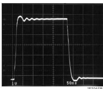
Large-Signal Transient ( A_V = -1 , C_L = 200pF )
