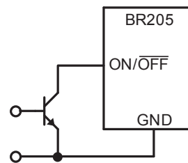
Figure 5. \text{ON}/\overline{\text{OFF}} peripheral circuit
