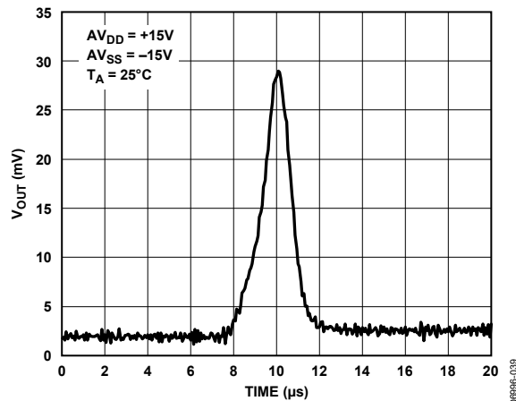
Figure 43. V_{OUT} vs. Time on Power-Up
