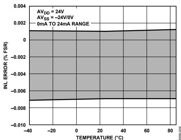
Figure 47. Integral Nonlinearity vs. Temperature, Internal R_{SET}
