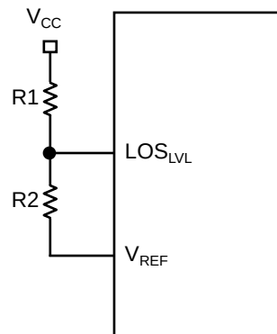
Figure 3. LOS_LVL Circuit
