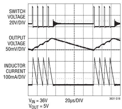
Operating Waveforms
