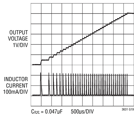
Soft-Start Waveforms
